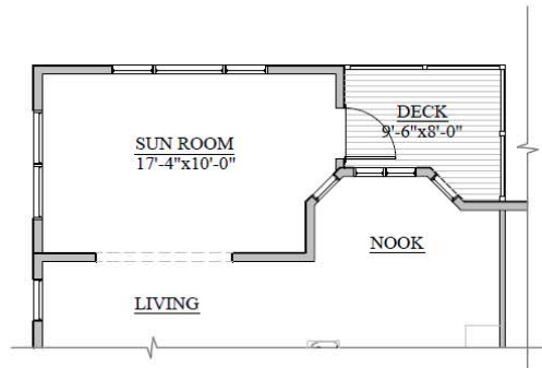
PARTIAL FLOOR PLAN
