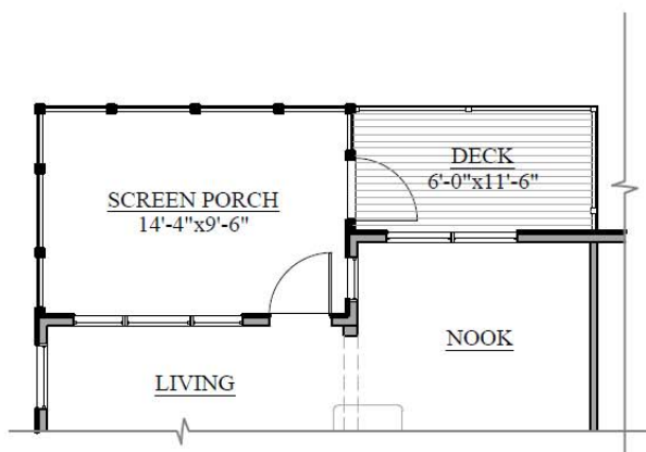
PARTIAL FLOOR PLAN
