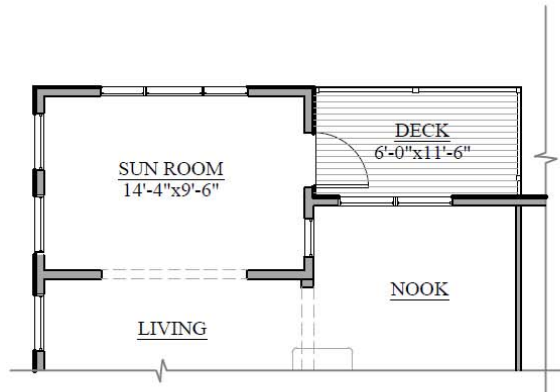
PARTIAL FLOOR PLAN
