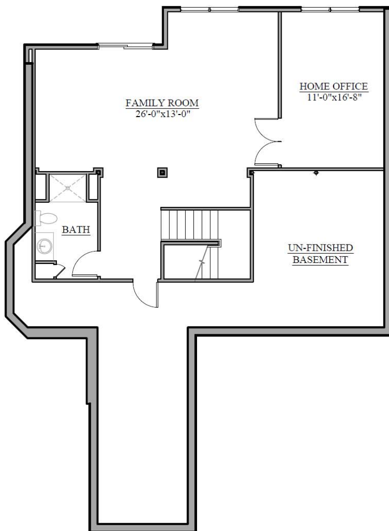
BASEMENT FLOOR PLAN 860 Square Feet Option #110
